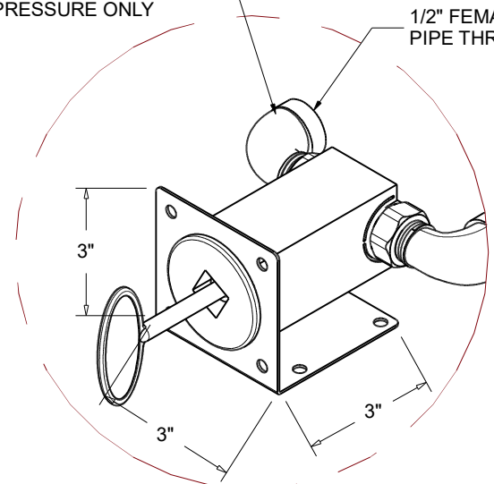
BRACKET DETAIL
